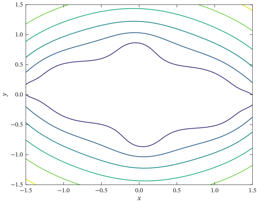
Isolines of \ln(1 + |z_3|)
