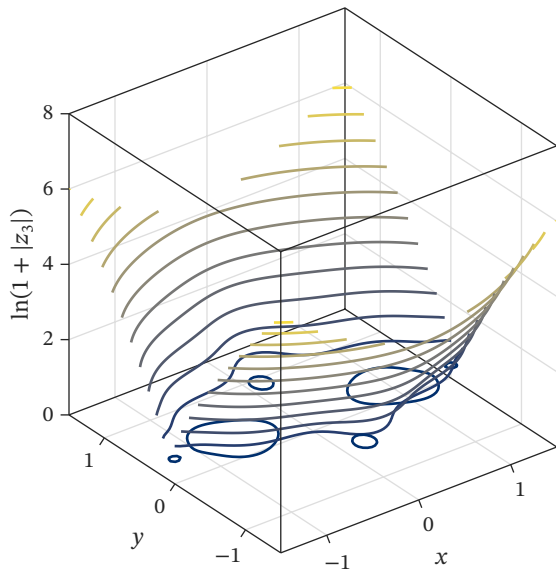
Isolines of \ln(1 + |z_3|) at their levels
