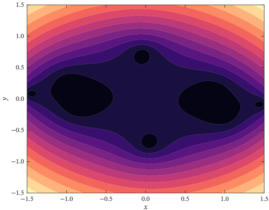
Filled contours of \ln(1 + |z_3|)
