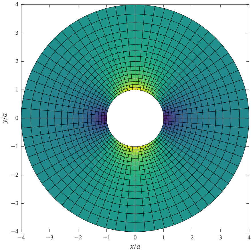
Speed |\mathbf{u}|/U_\infty of the potential flow past a cylinder
