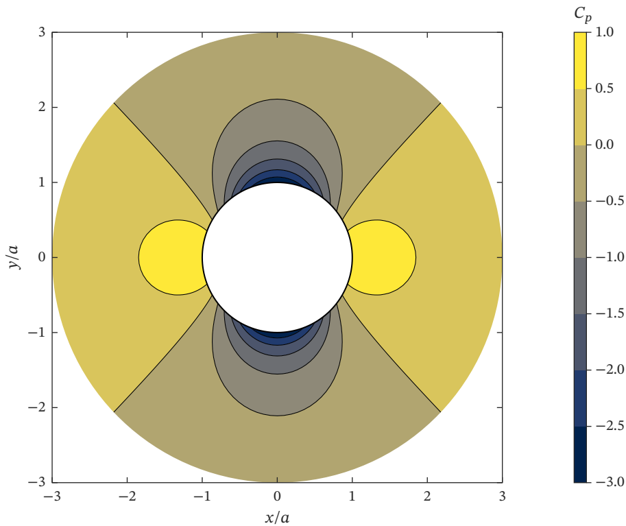
Pressure coefficient C_p of the potential flow past a cylinder
