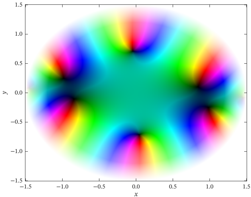
Domain colouring of z_3
