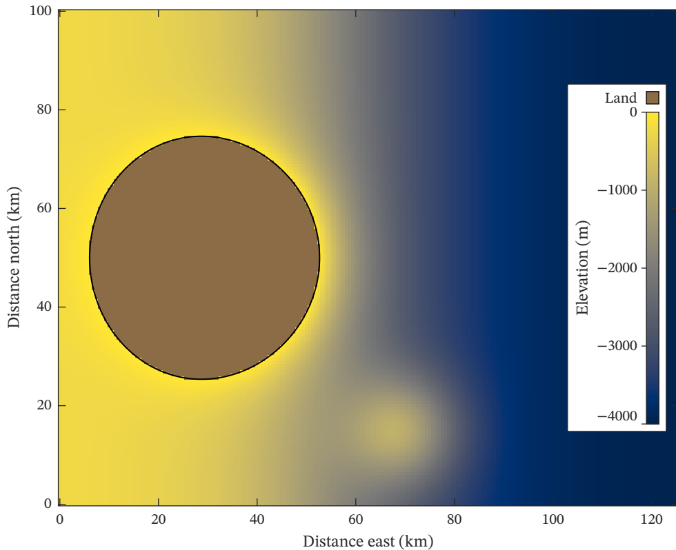
Bathymetry around a volcanic island
