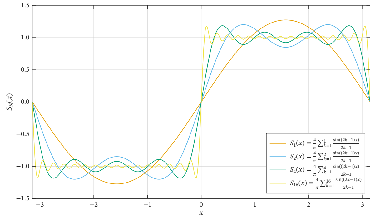
Fourier series of a square wave
