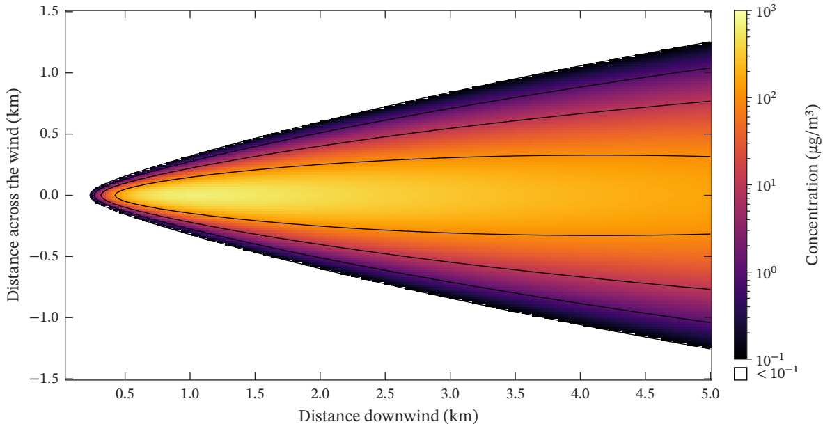
Ground-level concentration downwind of a 60 m stack
