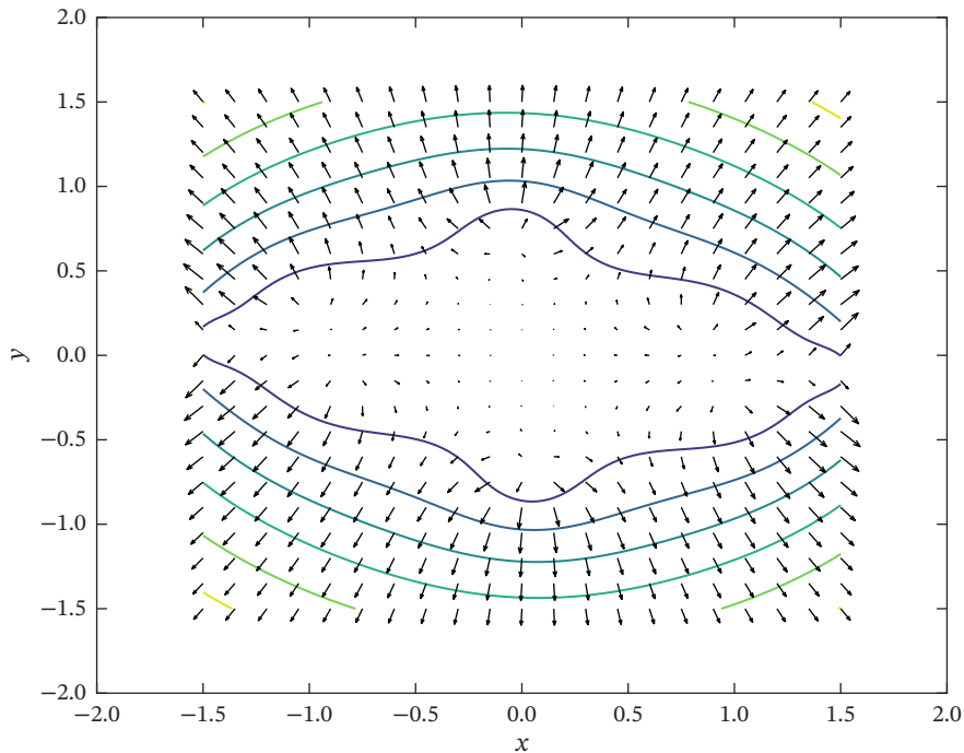
Gradient of \ln(1 + |z_3|)
