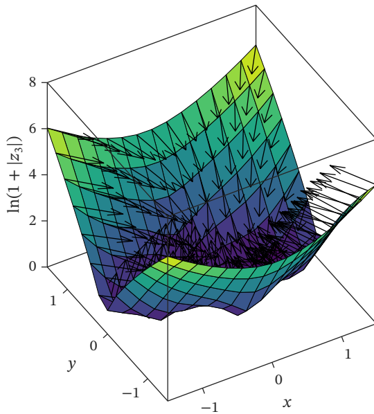
Normals of the surface of \ln(1 + |z_3|)
