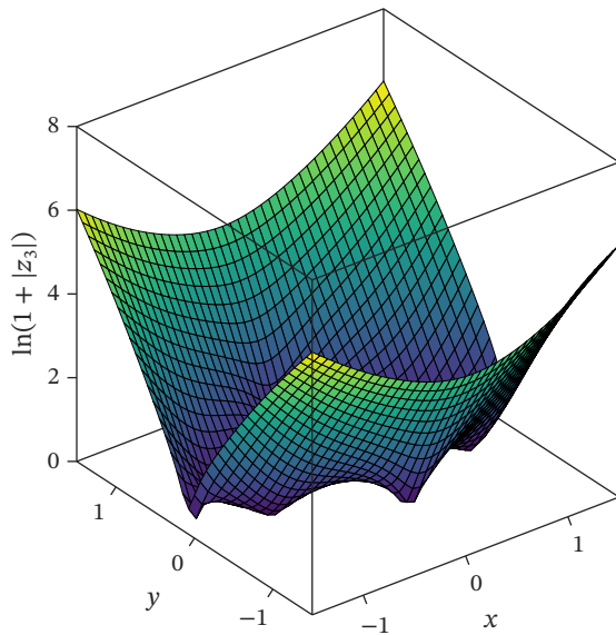
Surface of \ln(1 + |z_3|)
