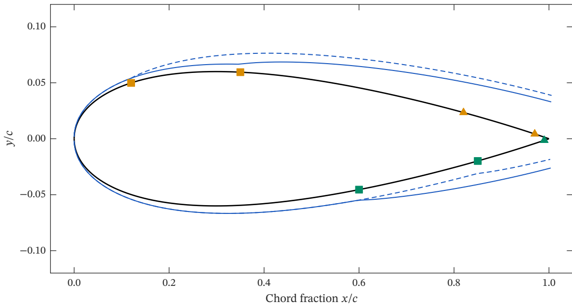
Boundary layer on a NACA 0012 section
